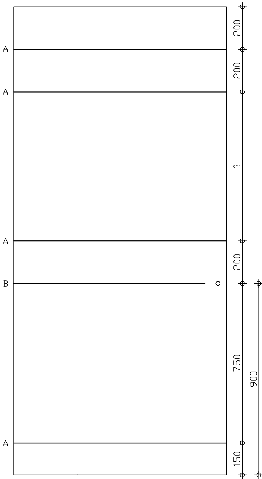
DETAIL Doorsnede trekker / Coupe tirant
