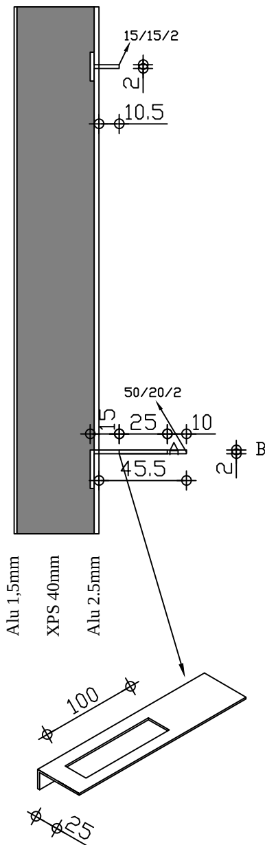
DETAIL Doorsnede trekker / Coupe tirant
